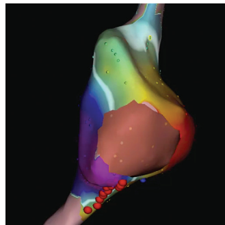
Electroanatomic map
